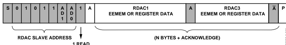
Figure 9. RDAC Current Read (Restricted to Previously Selected Address Stored in the Register).
