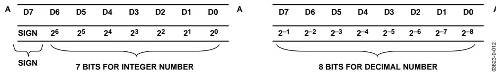
Figure 12. Format of Stored Tolerance in Sign Magnitude Format with Bit Position Descriptions. (Unit is percent. Only data bytes are shown.)
