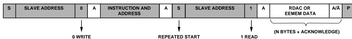
Figure 10. RDAC or EEMEM Random Read
