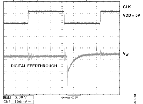
Figure 31. Clock Feedthrough and Midscale Transition Glitch
