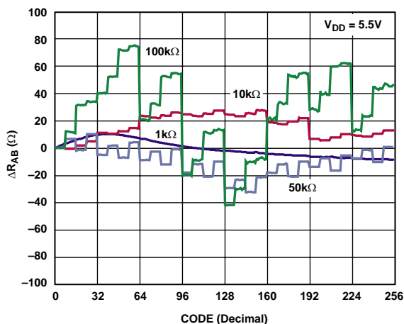
Figure 29. AD5252 \Delta R_{AB} vs. Code, T_A = 25^\circ\text{C}
