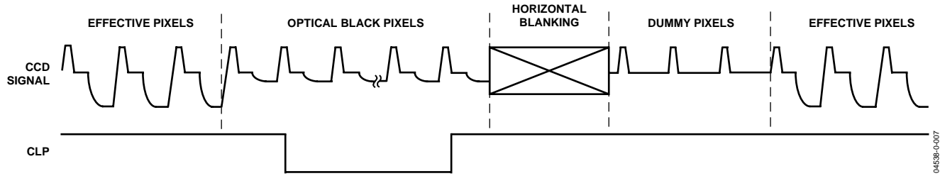
Figure 4. CLP Timing
