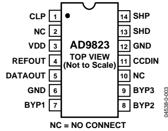
Figure 2. Pin Configurations
