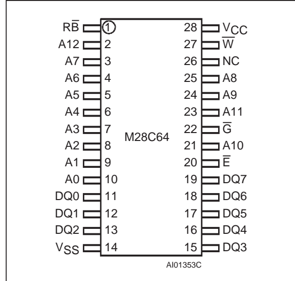
Figure 2C. SO Connections
