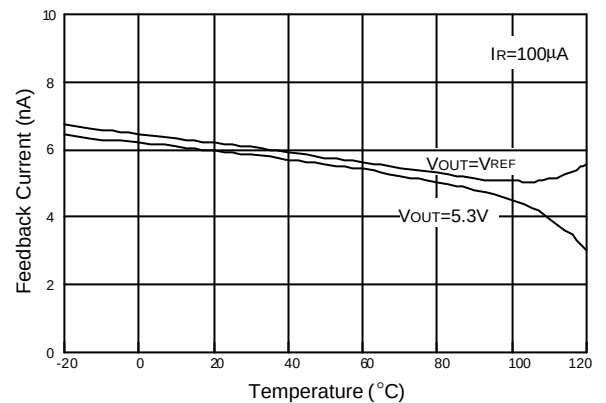
Fig. 6 Feedback Current
