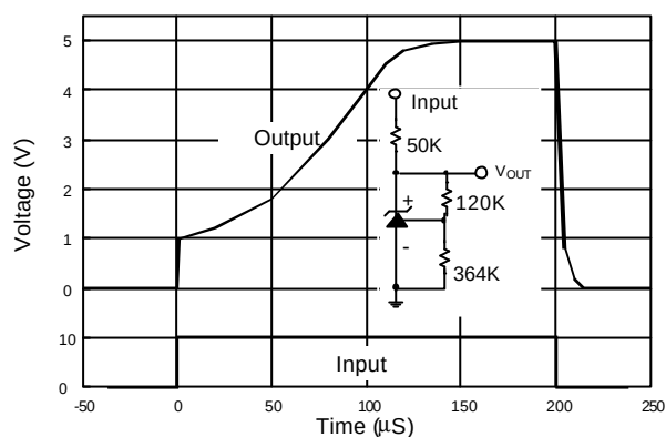
Fig. 7 Response Time
