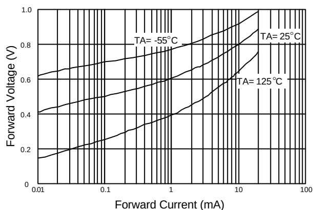
Fig. 1 Forward characteristics
