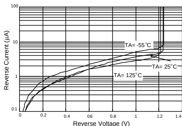
Fig. 2 Reverse Characteristics
