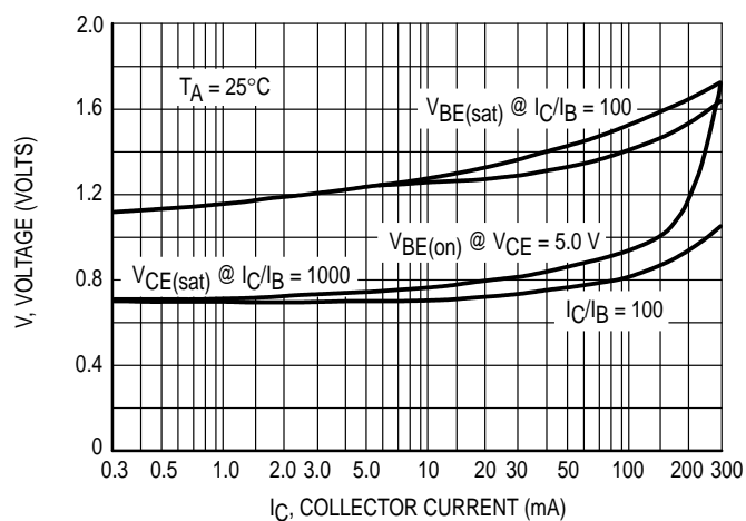
Figure 3. "On" Voltage
