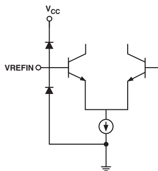
Figure 6. Reference Input
