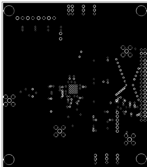
Figure 18. Ground Plane
