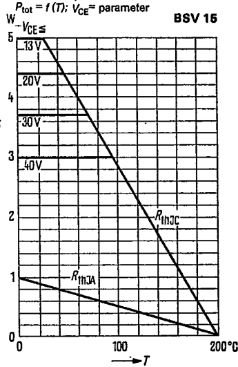
Total perm. power dissipation versus temperature
