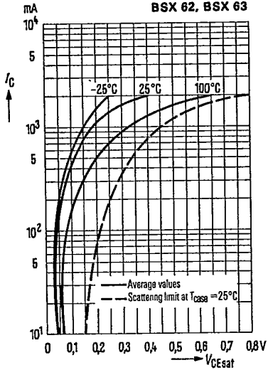
Collector-emitter saturation voltage V_{CEsat} = f(I_C) h_{FE} = 10 ; T_{amb} = \text{parameter} (common emitter configuration) BSX 62, BSX 63
