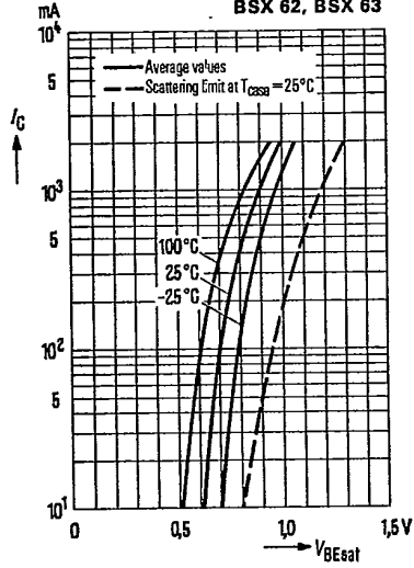
Collector-base saturation voltage V_{BEsat} = f(I_C) h_{FE} = 10 ; T_{amb} = \text{parameter} (common emitter configuration) BSX 62, BSX 63
