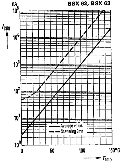
Collector cutoff current versus temperature I_{CBO} = f(T_{amb}) BSX 62, BSX 63
