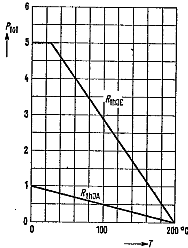
Total perm. power dissipation versus temperature W P_{tot} = f(T); R_{th} = \text{parameter}
