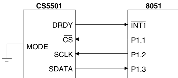
Figure A6. MCS51 (8051) /CS5501 Serial Interface
