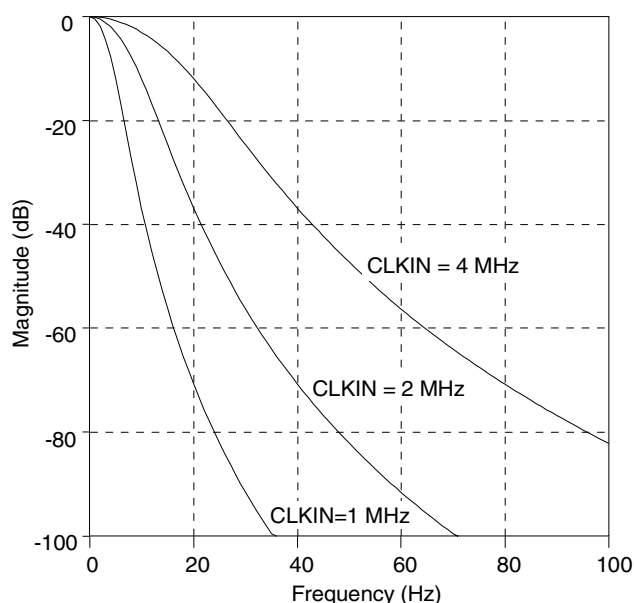
b. 6-Pole Gaussian Filter Response
