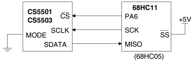
Figure A3. 68HC11/CS5501 Serial Interface
