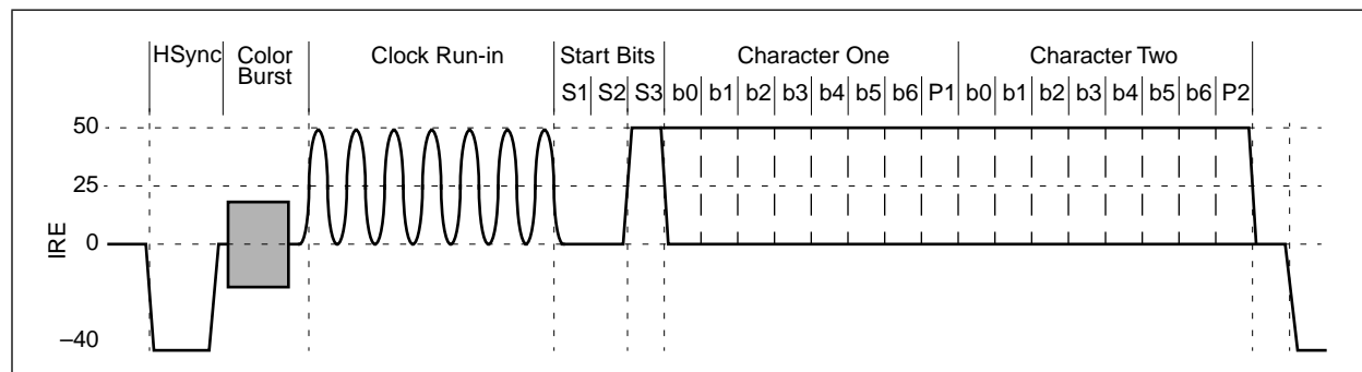
Figure 1-24. CC/EDS Incoming Signal
