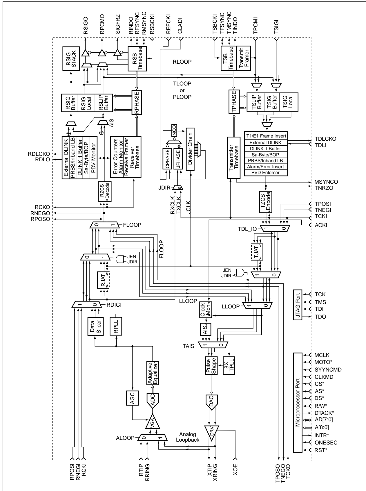
Figure 2-3. Detailed Bt8376 Block Diagram
