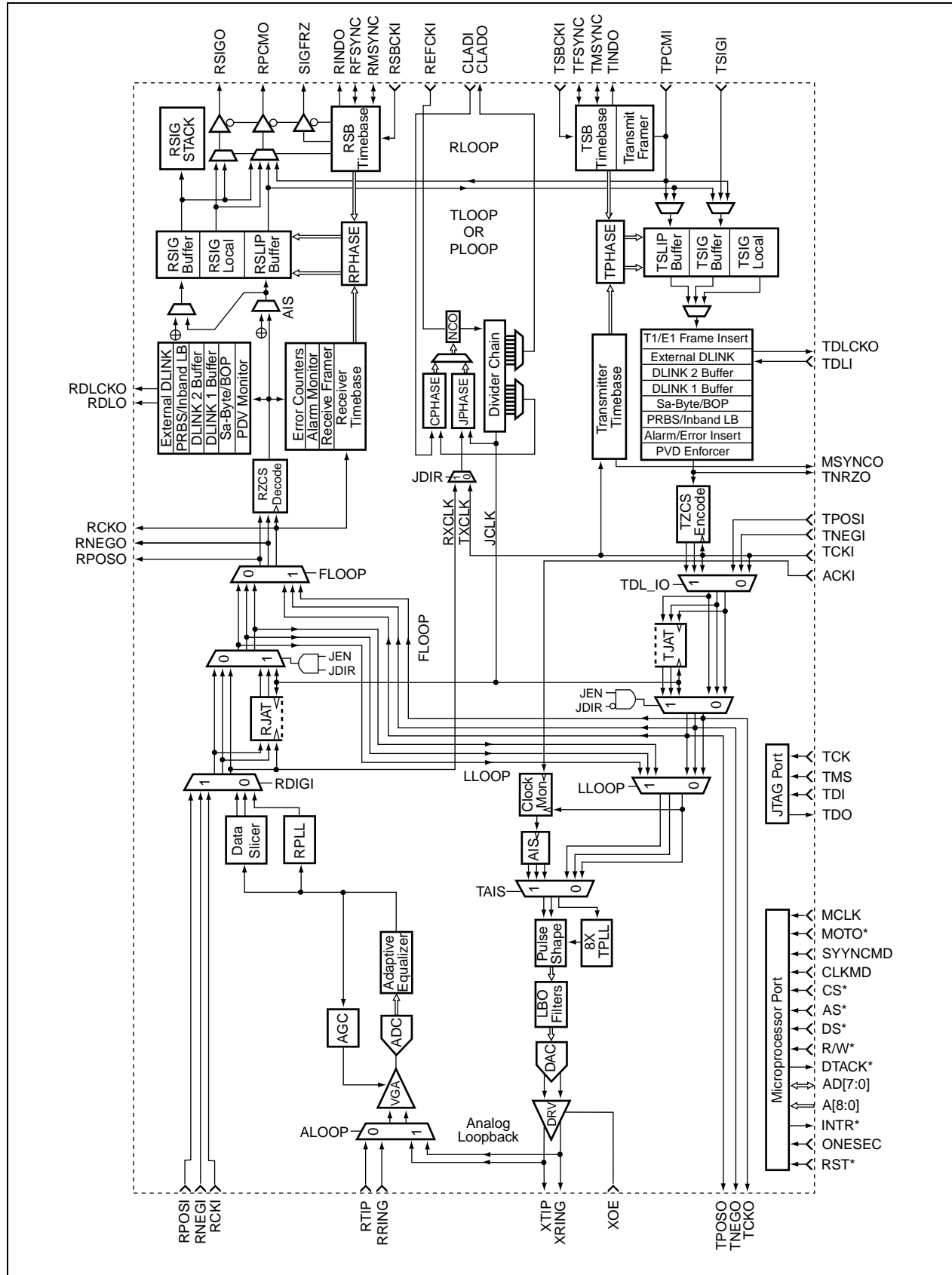
Figure 2-1. Detailed Bt8370 Block Diagram
