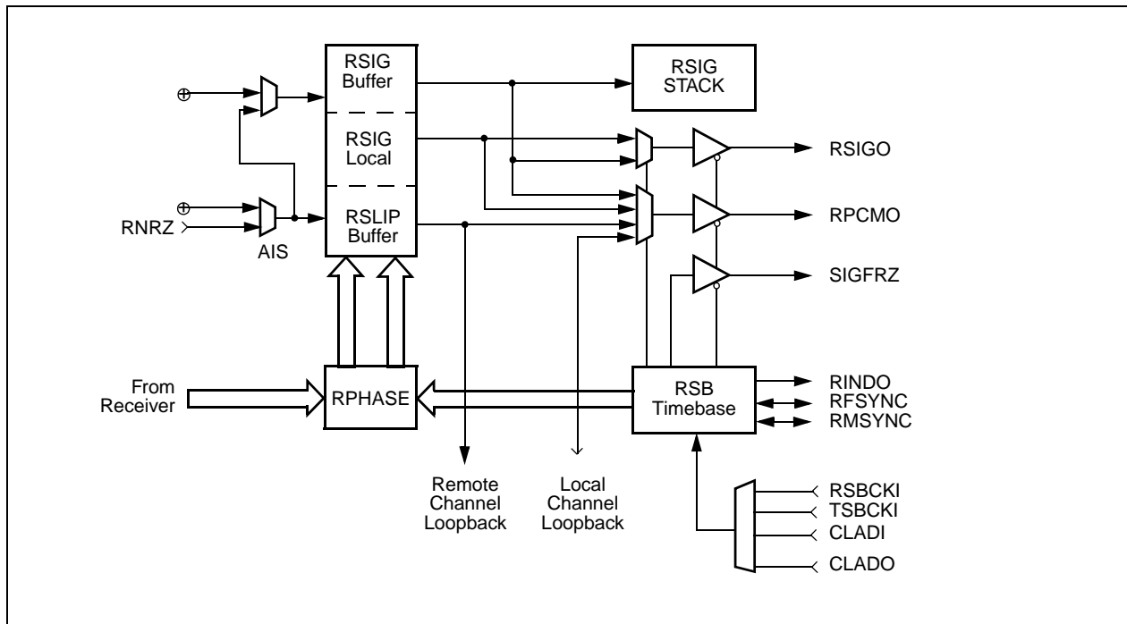
Figure 2-18. RSB Diagram
