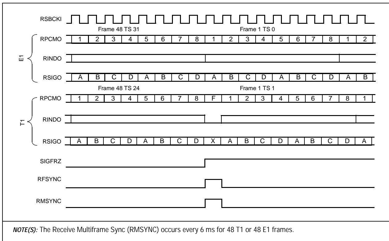
Figure 2-15. RSB Waveforms
