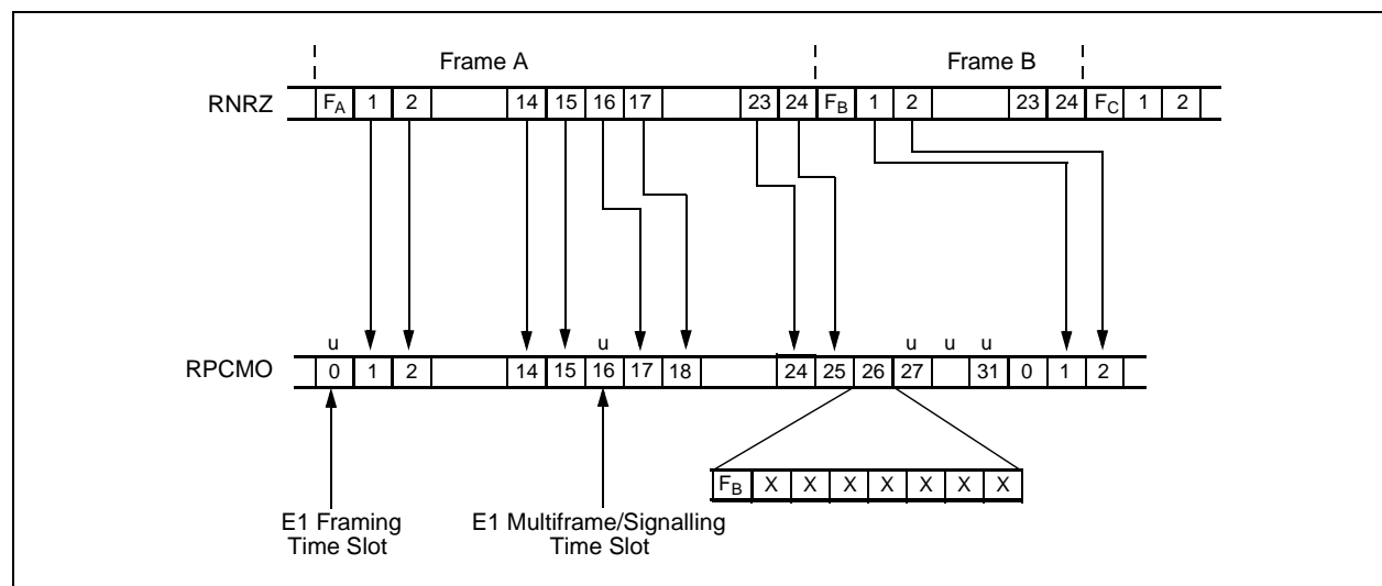
Figure 2-20. G.802 Embedded Framing
