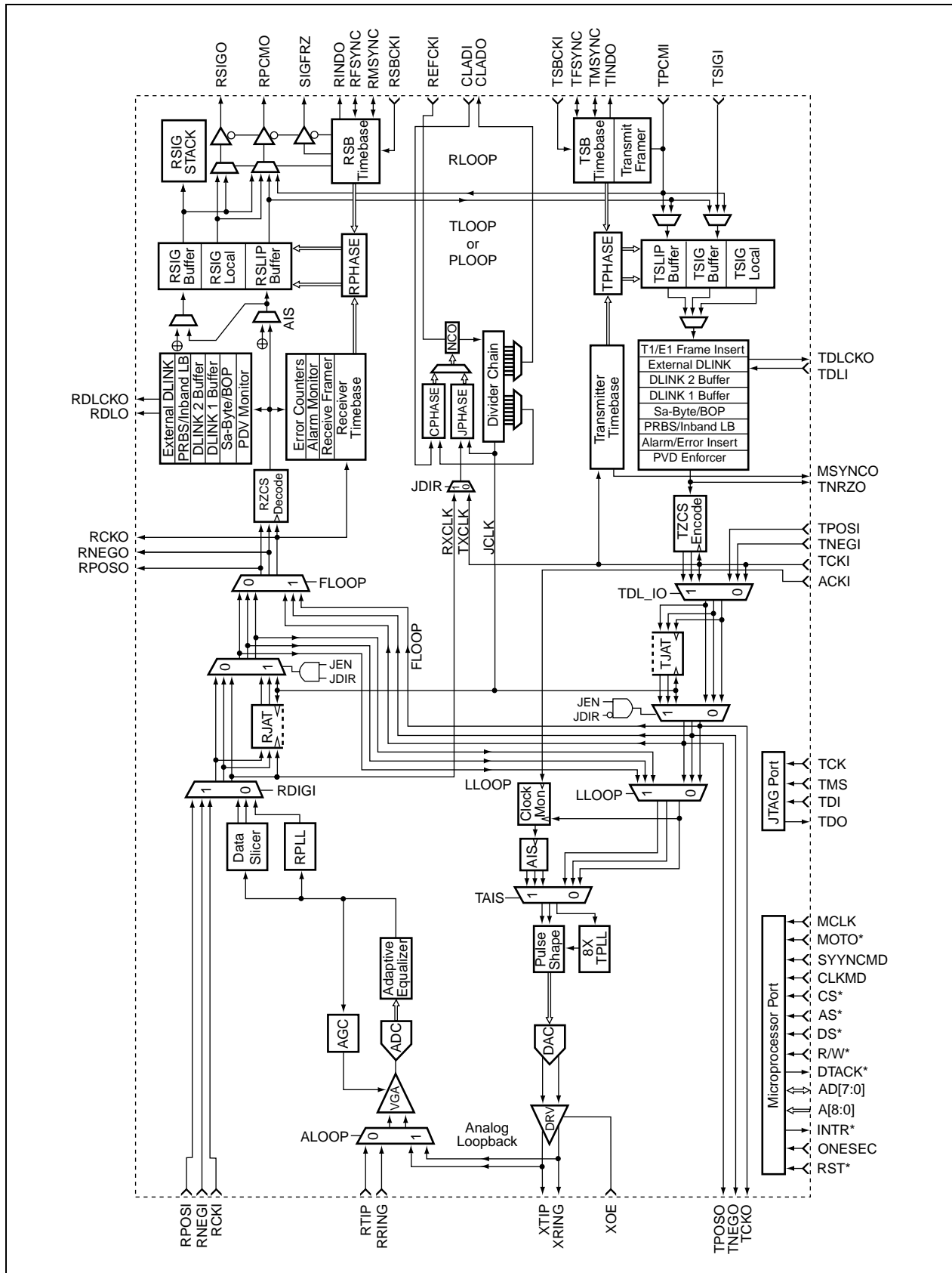
Figure 2-2. Detailed Bt8375 Block Diagram
