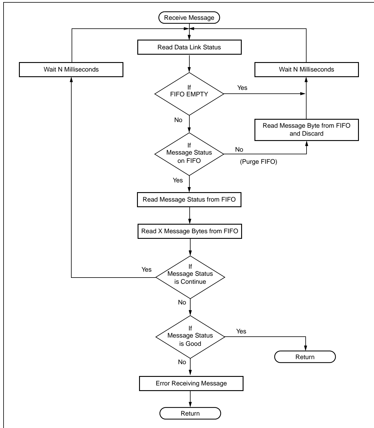
Figure 2-13. Polled Receive Data Link Processing
