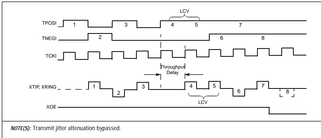
Figure 2-34. TLIU Waveform
