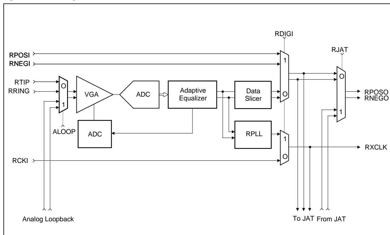
Figure 2-4. RLIU Diagram
