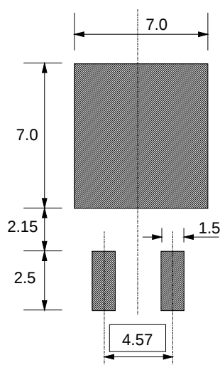
Fig.13. SOT428 : minimum pad sizes for surface mounting.
