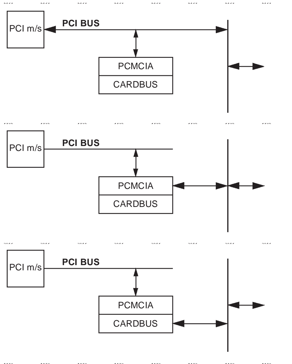
Figure 1.2. PCI, PCMCIA &amp; CARDBUS modes:
