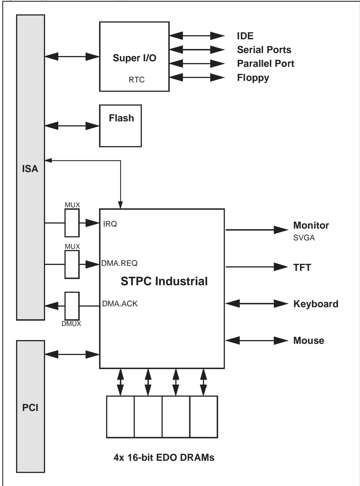
Figure 2. Typical PC oriented Application
