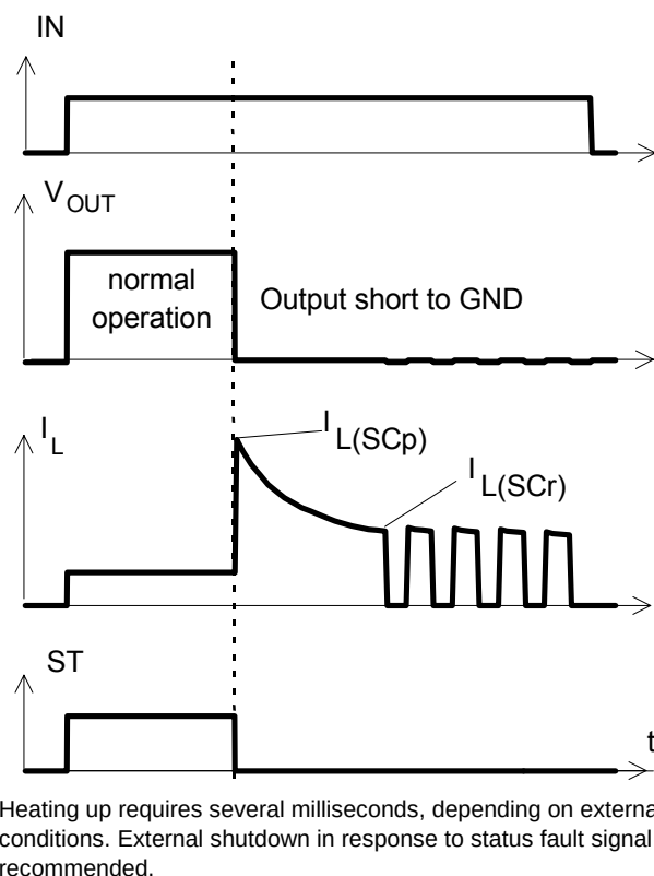
Figure 4a: Overtemperature: Reset if T_j < T_{jt}
