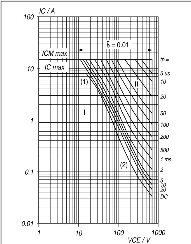
Fig. 15. Forward bias safe operating area. T_{mb} = 25^\circ C
