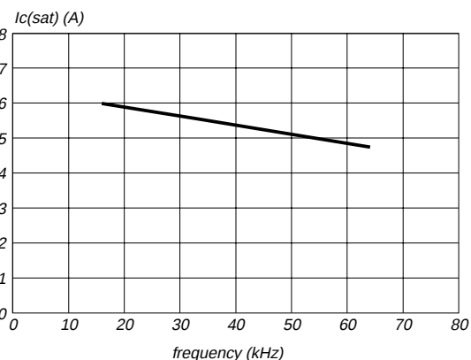
Fig.14. I_{C\text{sat}} during normal running vs. frequency of operation for optimum performance
