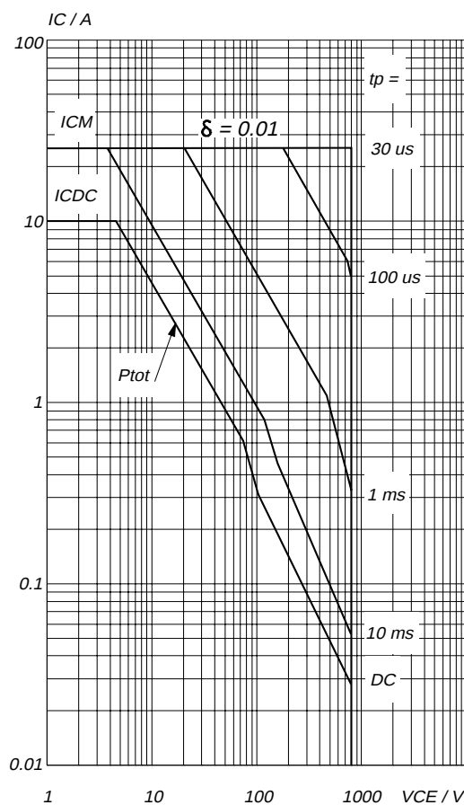
Fig.13. Forward bias safe operating area. T_{hs} = 25^\circ\text{C} I_{CDC} & I_{CM} = f(V_{CE}) ; I_{CM} single pulse; parameter t_p Second-breakdown limits independent of temperature. Mounted with heatsink compound.
