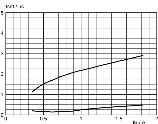
Fig.10. Typical collector storage and fall time. ts = f(I_B) ; tf = f(I_B) ; I_C = 5.5\text{ A} ; T_j = 85^\circ\text{C} ; f = 64\text{ kHz}
