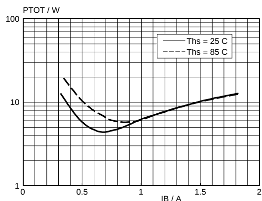
Fig.9. Typical losses. P_{TOT} = f(I_B) ; I_C = 5.5\text{ A} ; f = 64\text{ kHz}
