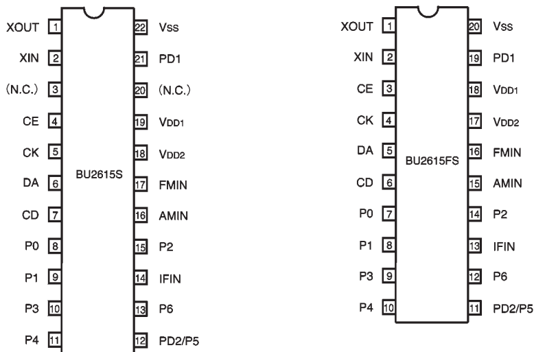
Fig.1 Pin assignments
