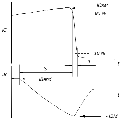
Fig.2. Switching times definitions.
