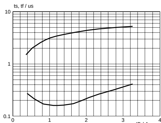
Fig.8. Limit storage and fall time. t_s = f(I_B) ; t_f = f(I_B) ; T_{HS} = 85^\circ\text{C} ; f = 64\text{ kHz}
