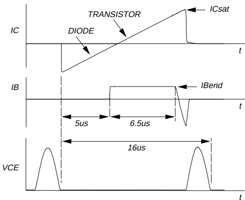
Fig.1. Switching times waveforms (64 kHz).
