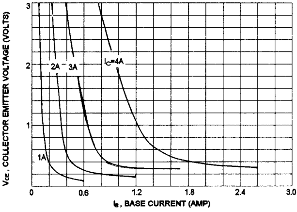
COLLECTOR-EMITTER VOLTAGE
