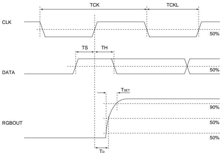
Fig. 2 Input / output interface timing
