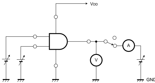
Fig. 1 DC characteristics
