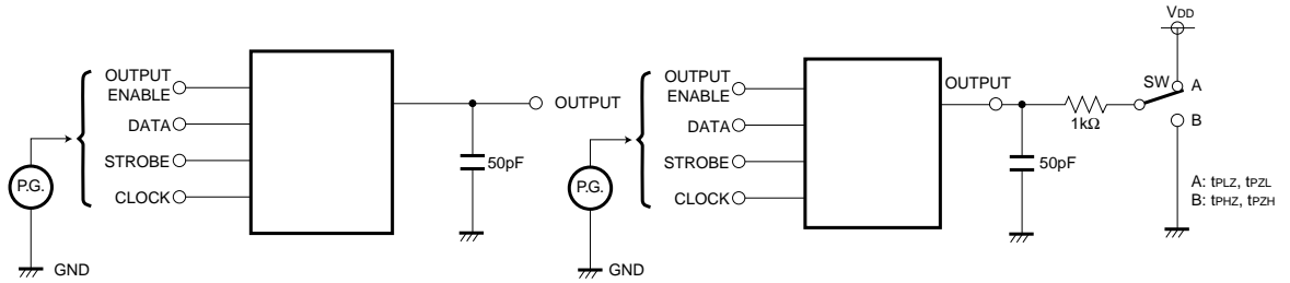
Fig. 1 Switching waveform
