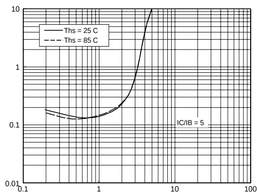
Fig.7. Typical collector-emitter saturation voltage.
