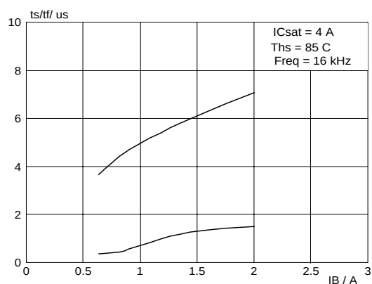
Fig.9. Typical collector storage and fall time. I_C = 4\text{ A} ; T_J = 85^\circ\text{C} ; f = 16\text{ kHz}
