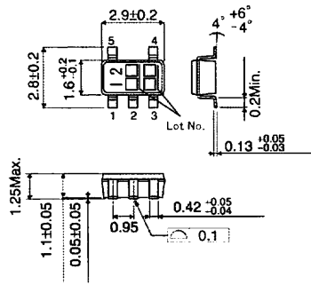
BU4S01G2(SSOP5)(UNIT:[mm])
