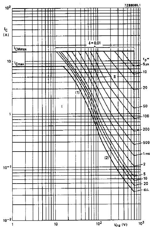
Fig.10. Forward bias safe operating area. T_{hs} < 25^{\circ}\text{C}
