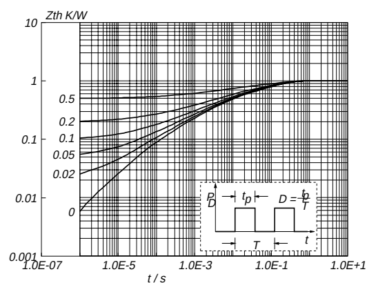
Fig.8. Transient thermal impedance. Z_{th\text{ j-hs}} = f(t) ; parameter D = t_p/T
