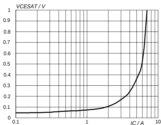
Fig.5. Typical collector-emitter saturation voltage. V_{CE\text{sat}} = f(I_C) ; parameter I_C/I_B
