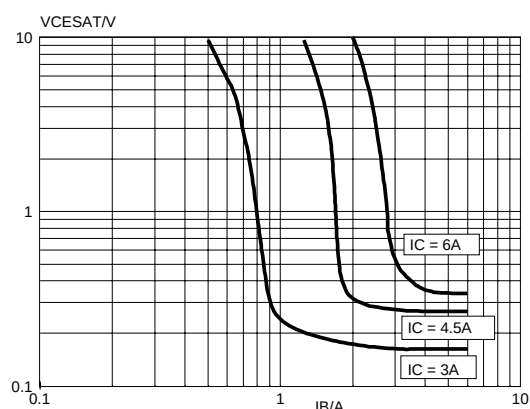
Fig.7. Typical collector-emitter saturation voltage. V_{CE\text{sat}} = f(I_B) ; parameter I_C
