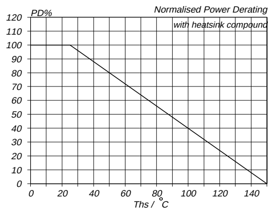
Fig.9. Normalised power dissipation. PD\% = 100 \cdot P_D / P_{D\ 25^\circ\text{C}} = f(T_{hs})
