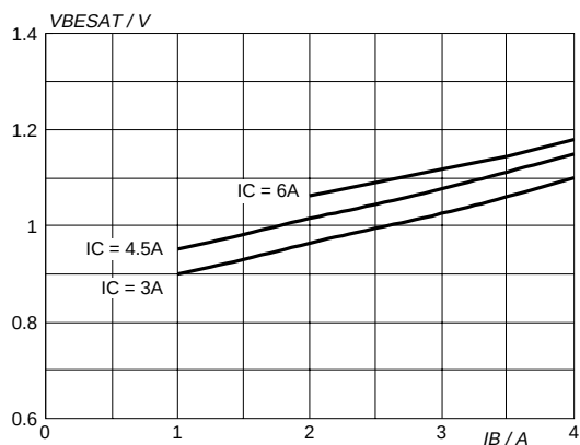
Fig.6. Typical base-emitter saturation voltage. V_{BE\text{sat}} = f(I_B) ; parameter I_C
