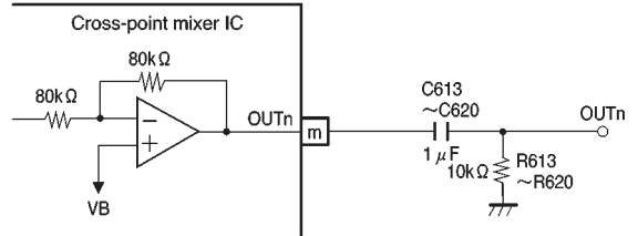
Fig. 7 Output circuit
