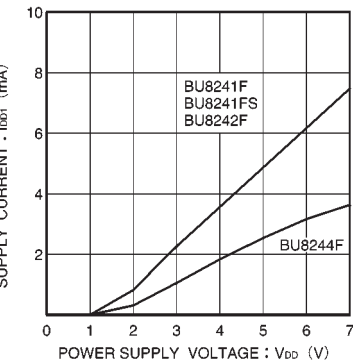
Fig. 9 Supply current vs. power supply voltage
