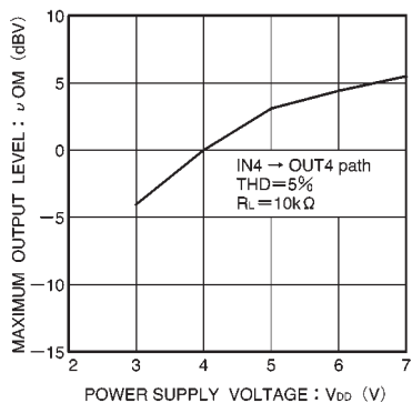
Fig. 12 Maximum output level vs. power supply voltage
