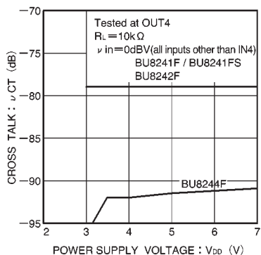
Fig. 15 Crosstalk vs. power supply voltage
