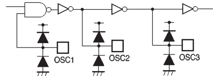
Oscillation circuit input/output
