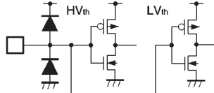
CMOS Schmitt trigger input
