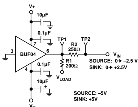
Figure 34. Transient Output Load Current Test Circuit
