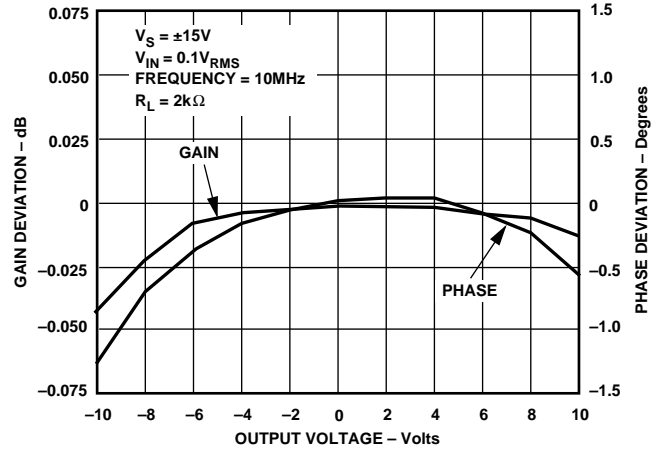
Figure 24. Gain and Phase Deviation, R_L = 2 k\Omega
