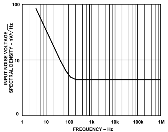
Figure 17. Input Noise Voltage vs. Frequency
