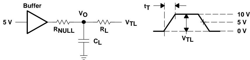
Figure 3. Transient Load Regulation Test Circuit
