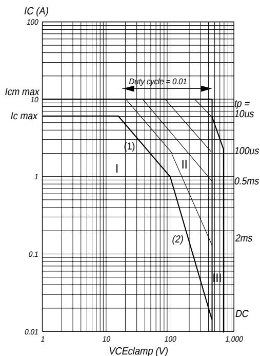
Fig.15. Forward bias safe operating area. T_{hs} \leq 25^\circ\text{C}
