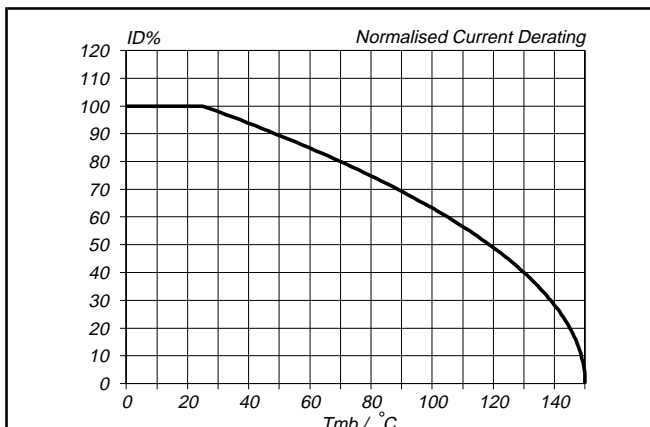
Fig.3. Normalised continuous drain current. I_D\% = 100 \cdot I_D / I_D(25^\circ C) = f(T_{mb}) ; conditions: V_{IS} = 5 V
