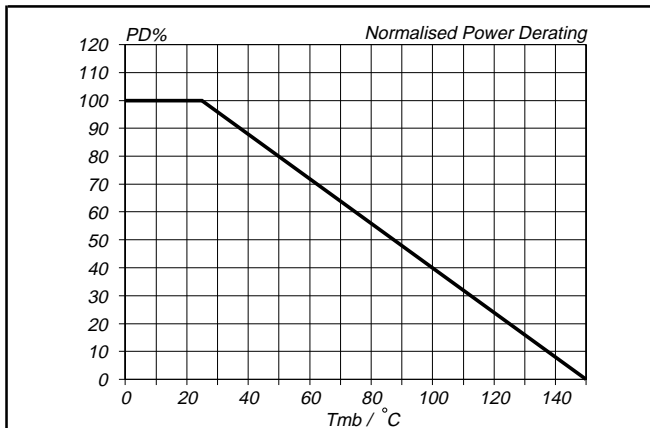
Fig.2. Normalised limiting power dissipation. P_D\% = 100 \cdot P_D / P_D(25^\circ C) = f(T_{mb})
