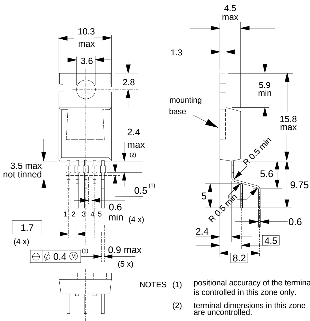
Fig.34. SOT263 leadform 263-01;
