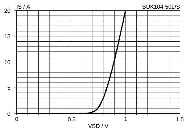
Fig.25. Typical reverse diode current, T_J = 25 \text{ °C} . I_S = f(V_{SDS}) ; conditions: V_{IS} = 0 \text{ V} ; t_p = 250 \text{ μs}
