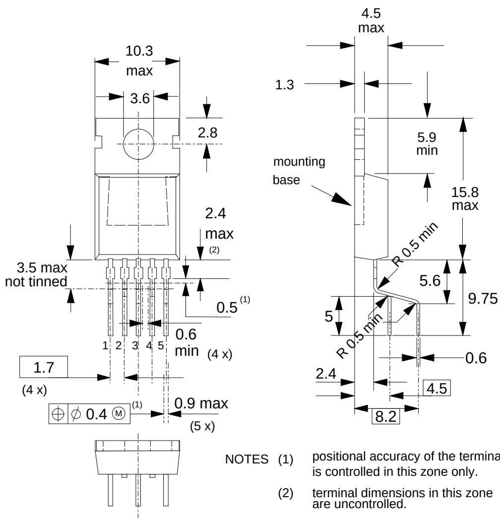
Fig.34. SOT263 leadform 263-01; pin 3 connected to mounting base.
