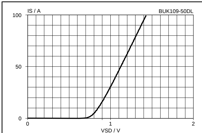
Fig.15. Typical reverse diode current, T_j = 25\text{ }^{\circ}\text{C} . I_S = f(V_{SDS}) ; conditions: V_{IS} = 0\text{ V}
