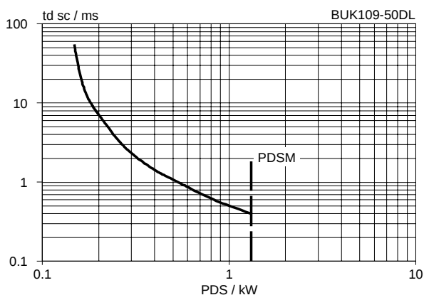
Fig.9. Typical overload protection characteristics. t_{d\text{sc}} = f(P_{DS}) ; conditions: V_{IS} \geq 4\text{ V} ; T_J = 25^\circ\text{C} .
