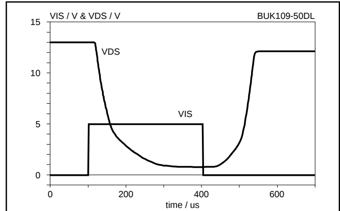
Fig.17. Typical switching waveforms, resistive load. V_{DD} = 13\text{ V} ; R_L = 2.1\text{ }\Omega ; R_I = 50\text{ }\Omega , T_j = 25\text{ }^{\circ}\text{C} .
