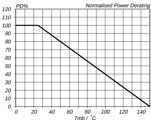
Fig.2. Normalised power dissipation. P_D\% = 100 \cdot P_D / P_D(25^\circ\text{C}) = f(T_{mb})
