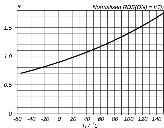
Fig.8. Normalised drain-source on-state resistance. a = R_{DS(ON)}/R_{DS(ON)25^\circ\text{C}} = f(T_J) ; I_D = 13\text{ A} ; V_{IS} = 5\text{ V}
