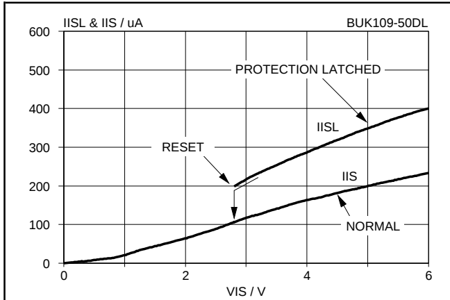
Fig.14. Typical DC input characteristics, T_j = 25\text{ }^{\circ}\text{C} . I_{ISL} & I_{IS} = f(V_{GS}) ; protection latched & normal operation
