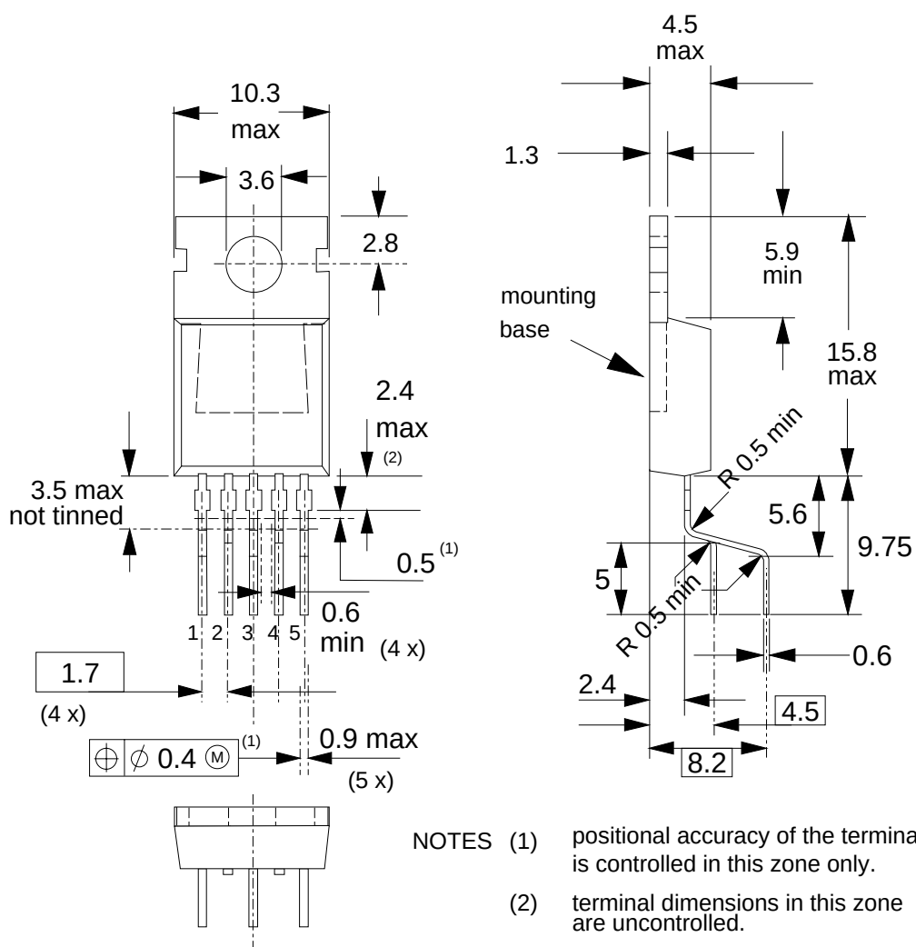
Fig.38. SOT263 leadform 263-01;
