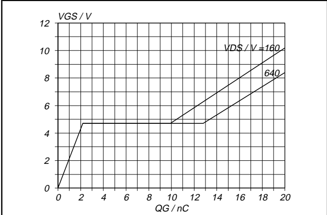
Fig.13. Typical turn-on gate-charge characteristics. V_{GS} = f(Q_G) ; conditions: I_D = 2.4 A; parameter V_{DS}
