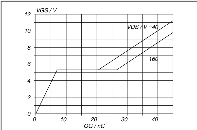
Fig.13. Typical turn-on gate-charge characteristics. V_{GS} = f(Q_G) ; conditions: I_D = 19 A ; parameter V_{DS}
