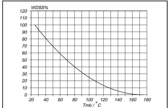
Fig.15. Normalised avalanche energy rating. W_{DSS}\% = f(T_{mb}) ; conditions: I_D = 26 A
