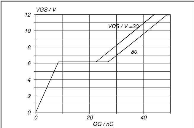
Fig.13. Typical turn-on gate-charge characteristics. V_{GS} = f(Q_G) ; conditions: I_D = 34 \text{ A} ; parameter V_{DS}
