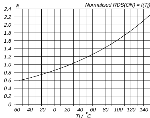
Fig.9. Normalised drain-source on-state resistance. a = R_{DS(ON)}/R_{DS(ON)25\text{ }^{\circ}\text{C}} = f(T_j) ; I_D = 3.5\text{ A} ; V_{GS} = 10\text{ V}
