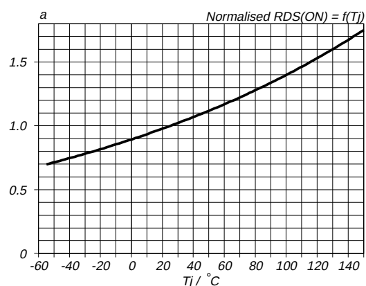
Fig. 9. Normalised drain-source on-state resistance. a = R_{DS(ON)}/R_{DS(ON)25\text{ }^{\circ}\text{C}} = f(T_j) ; I_D = 20\text{ A} ; V_{GS} = 10\text{ V}
