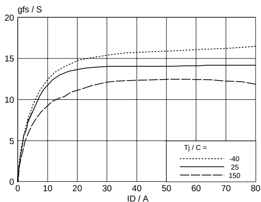
Fig. 8. Typical transconductance, T_j = 25\text{ }^{\circ}\text{C} . g_{fs} = f(I_D) ; conditions: V_{DS} = 15\text{ V}
