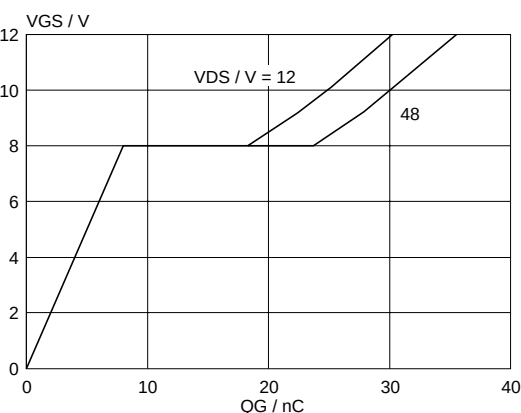
Fig.13. Typical turn-on gate-charge characteristics. V_{GS} = f(Q_G) ; conditions: I_D = 41\text{ A} ; parameter V_{DS}
