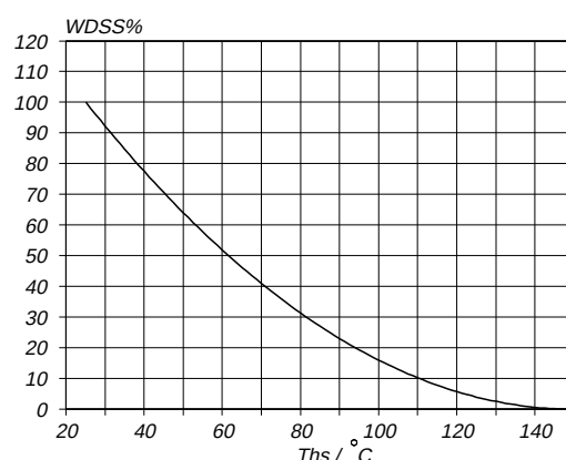
Fig.15. Normalised avalanche energy rating. W_{DSS}\% = f(T_{hs}) ; conditions: I_D = 41\text{ A}
