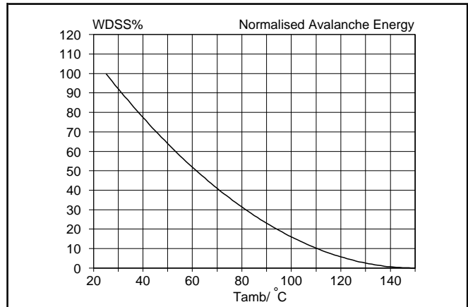
Fig.15. Normalised avalanche energy rating. W_{DSS}\% = f(T_{amb}) ; conditions: I_D = 1 A
