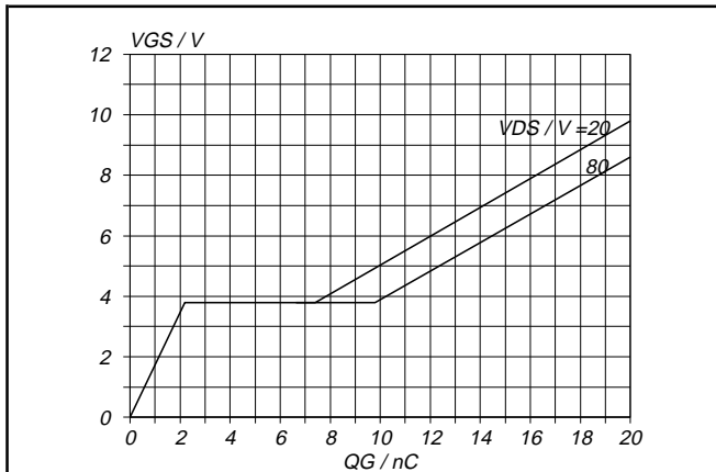
Fig.13. Typical turn-on gate-charge characteristics. V_{GS} = f(Q_G) ; conditions: I_D = 13 A; parameter V_{DS}
