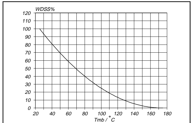
Fig.15. Normalised avalanche energy rating. W_{DSS}\% = f(T_{mb}) ; conditions: I_D = 13 A
