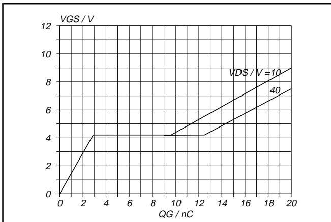
Fig. 13. Typical turn-on gate-charge characteristics. V_{GS} = f(Q_G) ; conditions: I_D = 20 A; parameter V_{DS}
