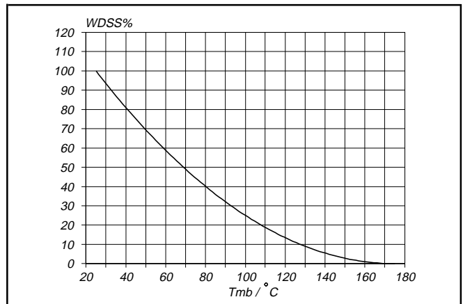
Fig. 15. Normalised avalanche energy rating. W_{DSS}\% = f(T_{mb}) ; conditions: I_D = 20 A
