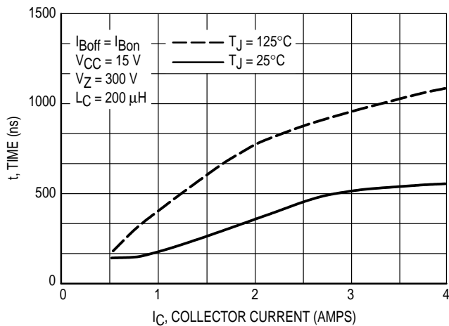
Figure 19. Inductive Switching, t_r @ I_C/I_B = 10
