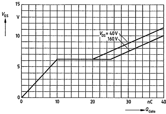
Typical gate-charge V_{GS} = f(Q_{Gate}) parameter: I_{D\ puls} = 14,3A
