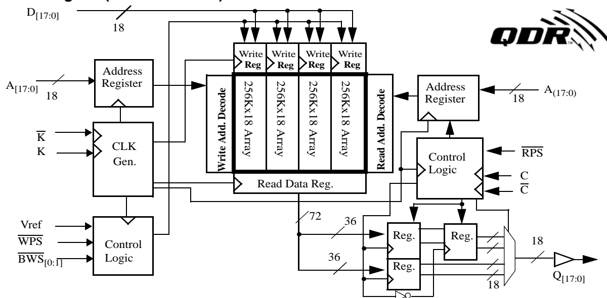
Logic Block Diagram (CY7C1305BV25)
