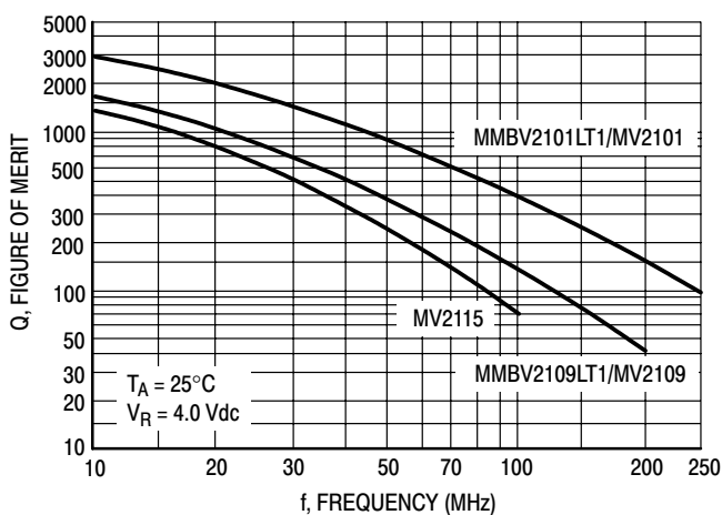
Figure 5. Figure of Merit versus Frequency
